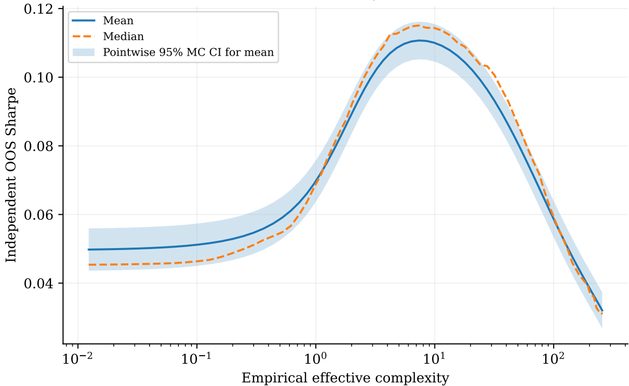
heteroskedastic, T=1440
